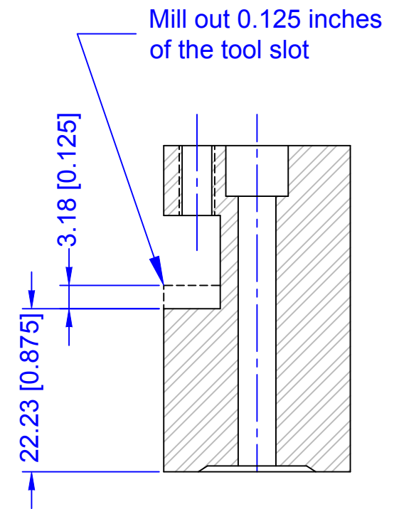
Front Tool Post for 3/8 Tools
