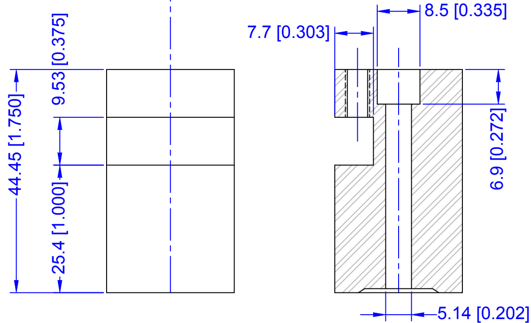
Taig Standard Front Tool Post
